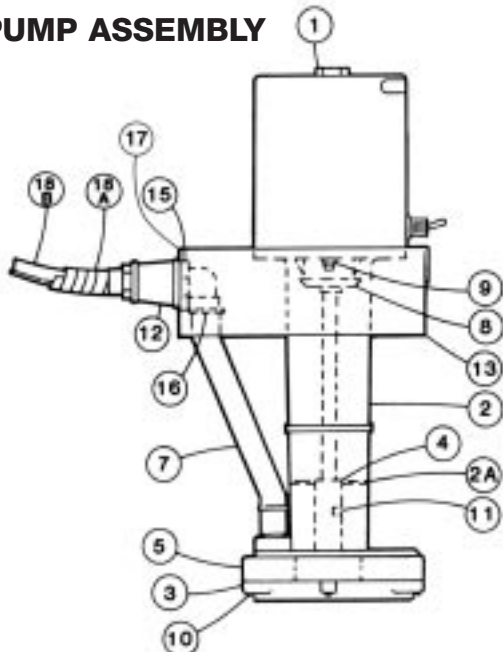
DETAIL "A"
