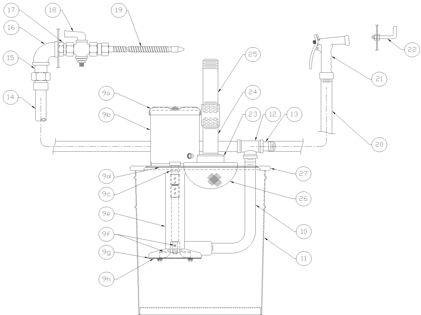
FLO-BAC PARTS WASHER
