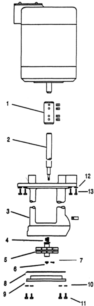
Exploded View
